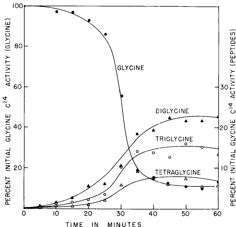
FIGURE 4 Homogeneous polypeptide formation by dicyandiamide.
