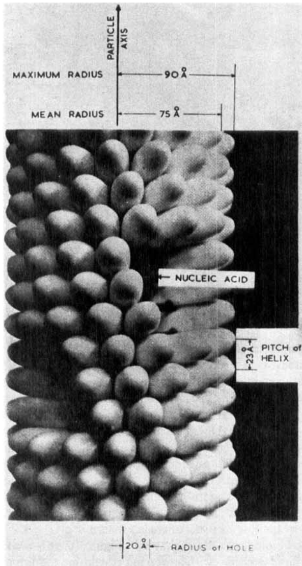
FIGURE 14 Diagrammatic structure of TMV.
