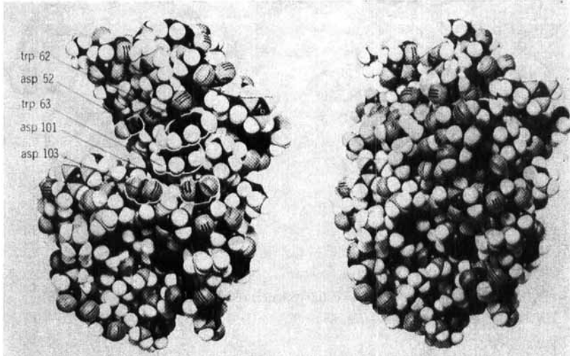
FIGURE 11 Structure of lysozyme showing substrate cleft.
