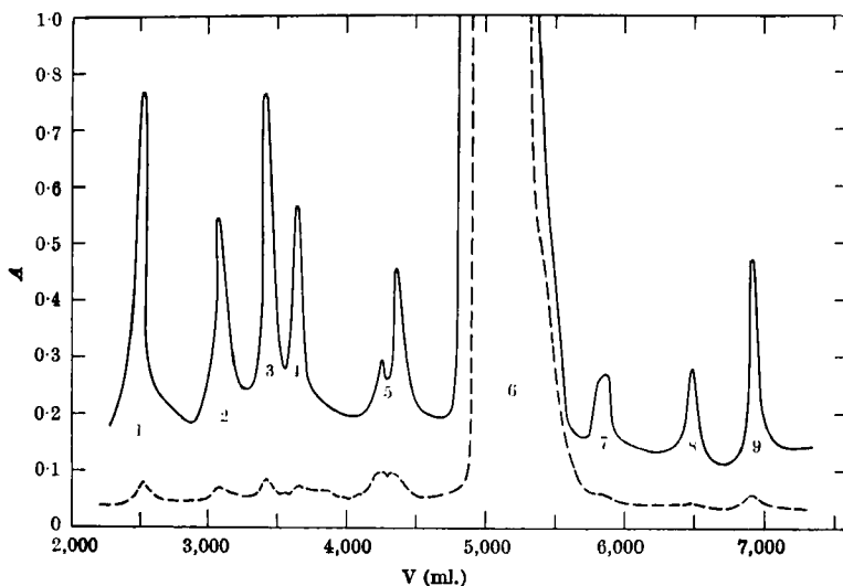
Chromatography of fraction II on 'Sephadex G-25', with gel bed 3 x 4 x 150 cm.
