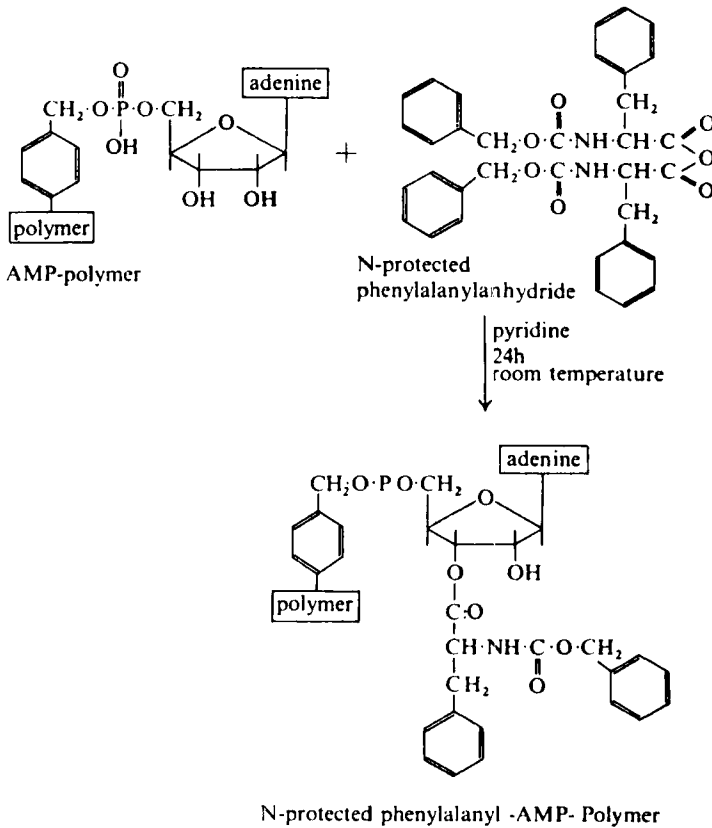
FIGURE 7 The coupling of the polymer-AMP complex with the anhydride form of an N-protected amino acid.
