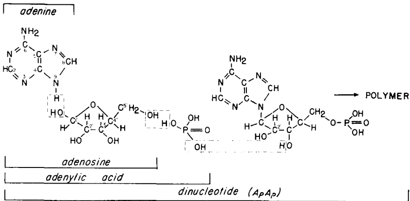
FIGURE 3 Dehydration condensation of polynucleotides.
